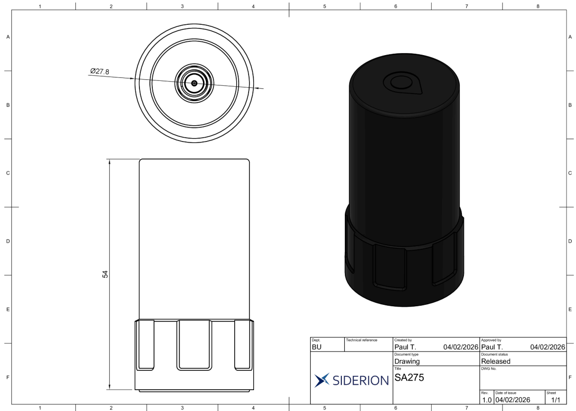
Figure 1. SA275 v1.0 mechanical drawings
